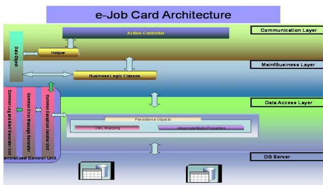
Figure 3 : application business components and the layers of the e-Job Card
