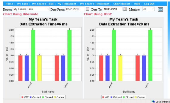
Figure 4 : Comparative study
