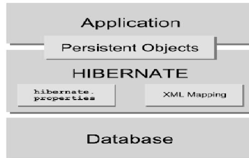
Figure 1 : Hibernate architecture
